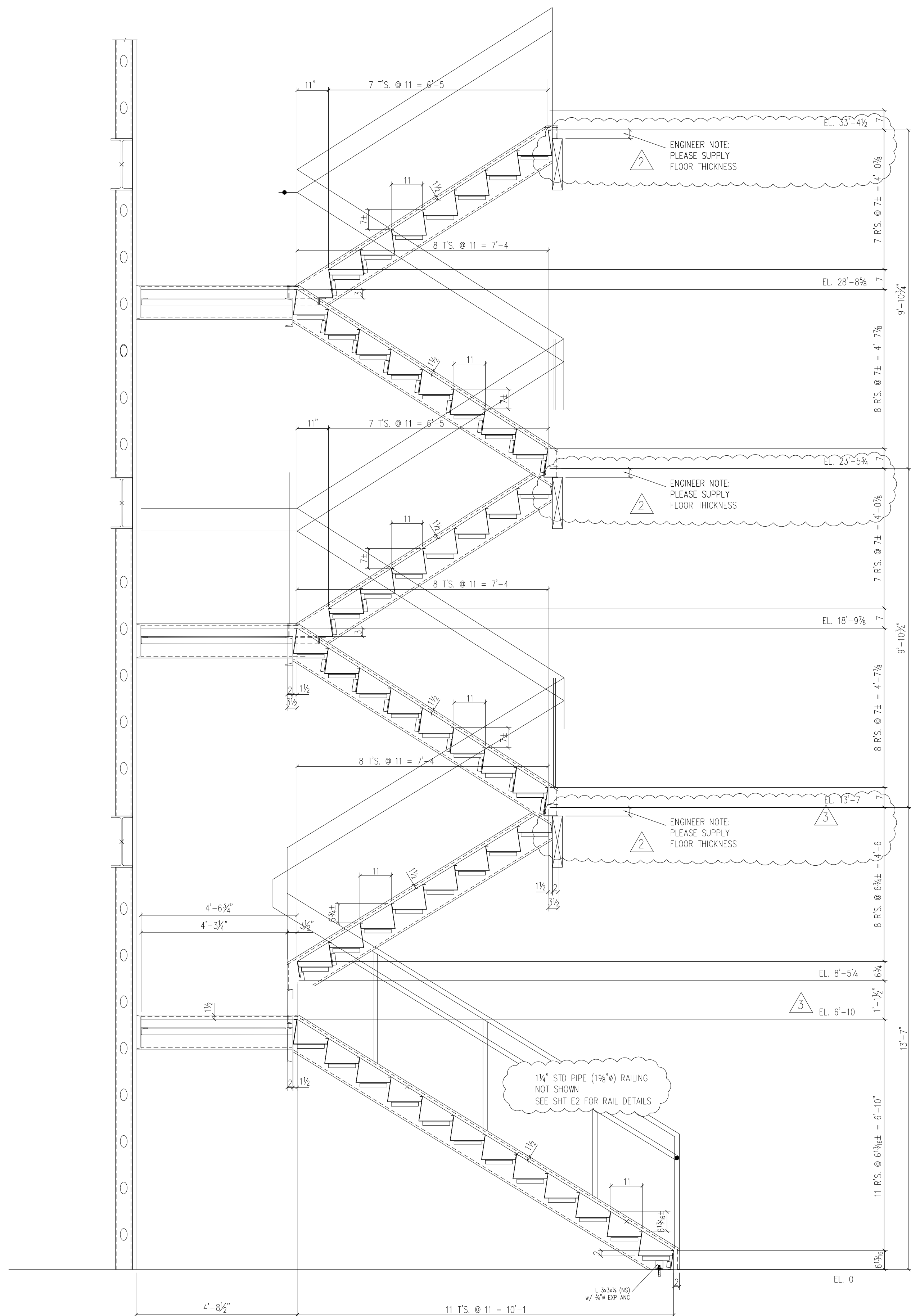
STAIR ELEVATION
